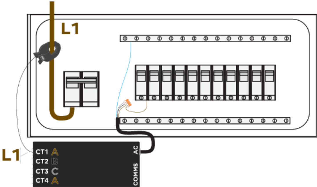
Figure 6. CT Measuring Single Phase System (CT on L1, Plugged into Port 1)
