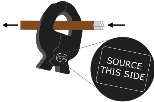
Figure 5. CT Orientation in Relation to Power Flow (Label to Face Power Source, in this Case Grid)
