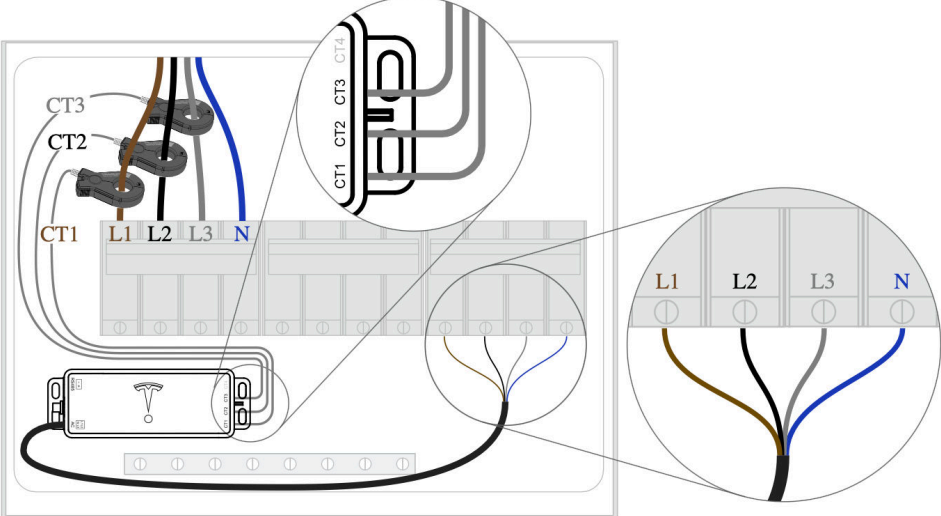
Figure 3. Configuration of remote meter inside panel - Three-phase
