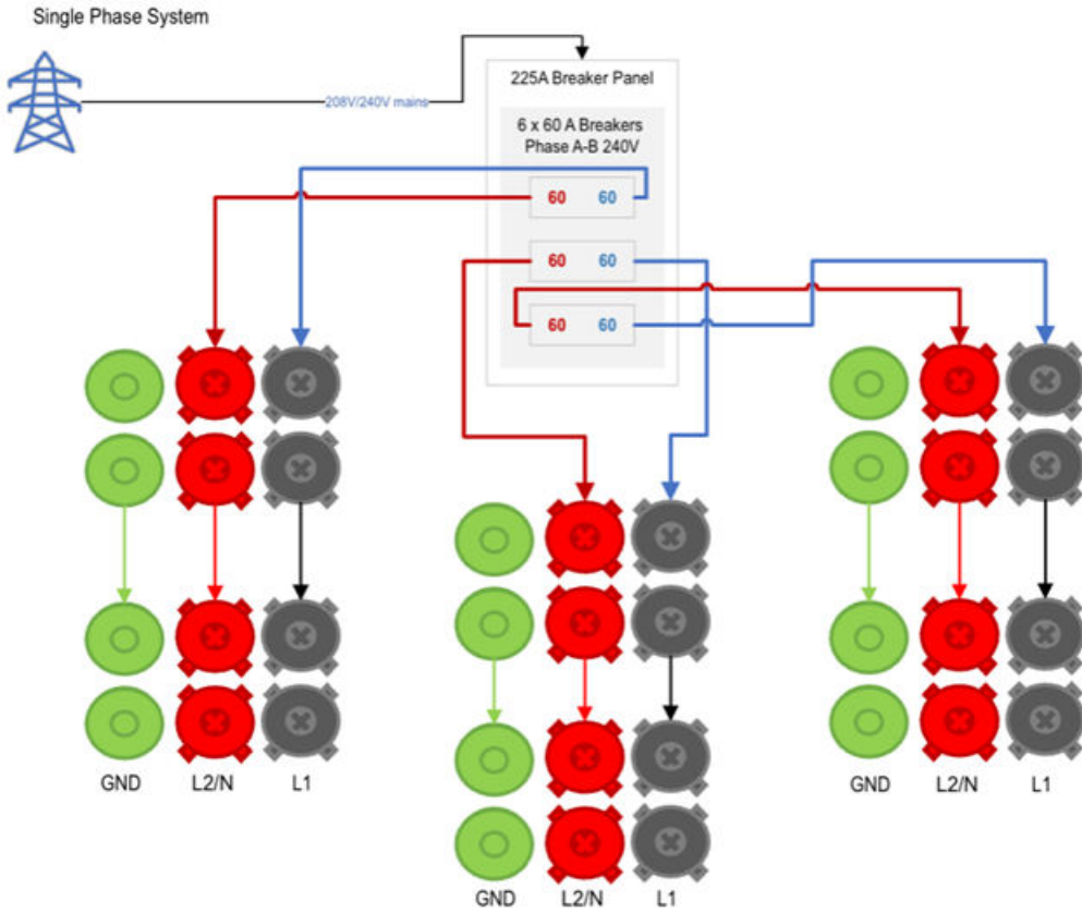
6 Wall Connector Daisy Chained 3 pairs
